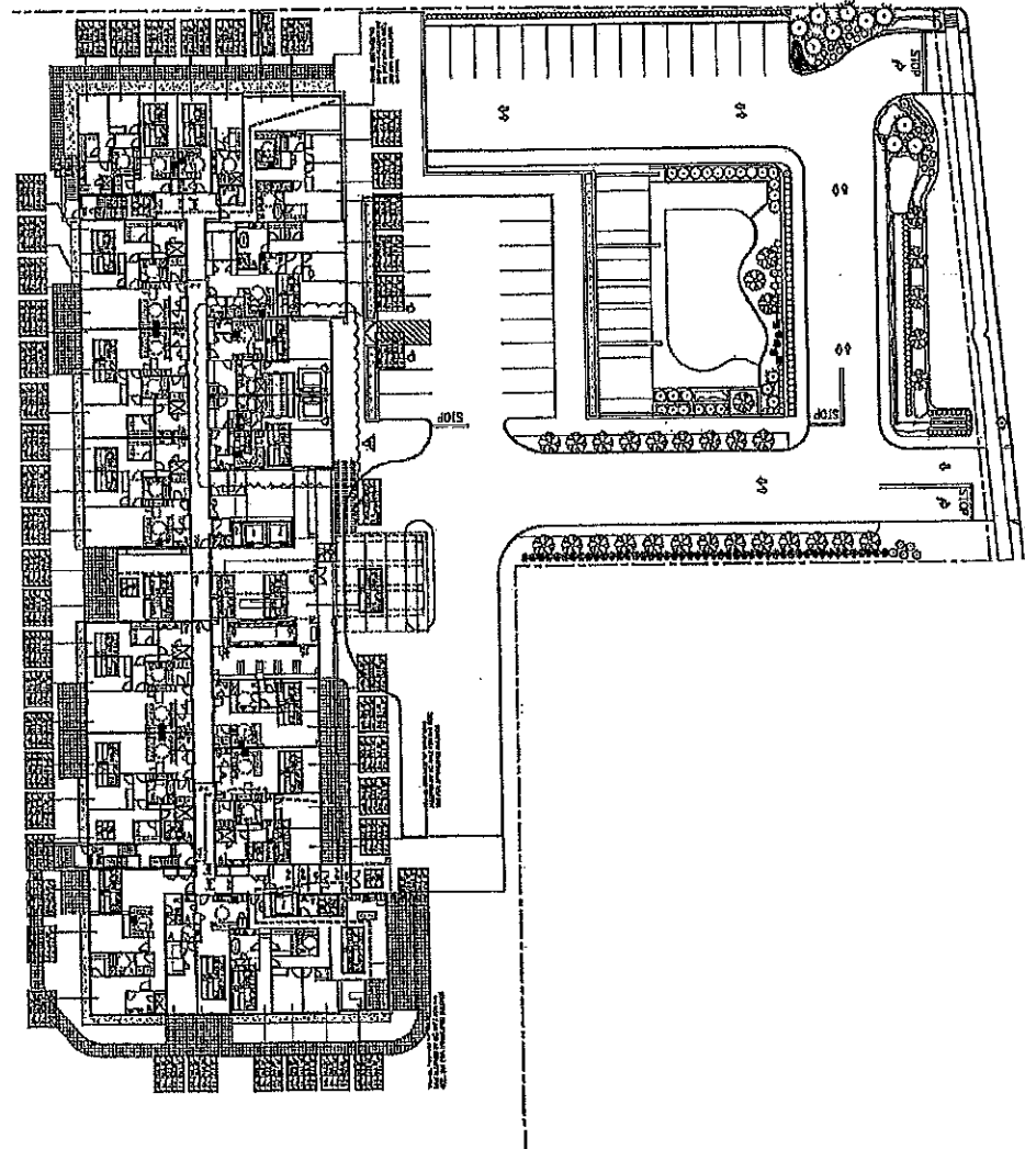
1. FIRST FLOOR EGRESS PLAN SCALE: 1/8" = 1'-0"
